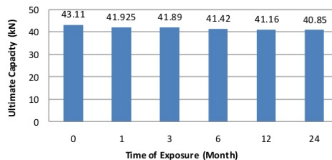
Fig.7. Ultimate capacity of beam specimens.
