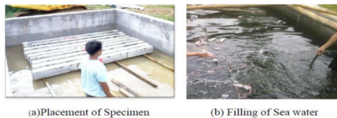
2 Fig.3. Preparation of concrete beams into sea water simulation pool
