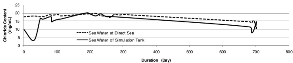
Fig.5 Control of Chloride content of sea water.
