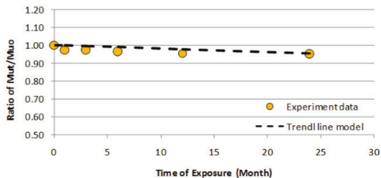
Fig.10. Trend of the M_{ut}/M_{u0} to the time of exposure.
